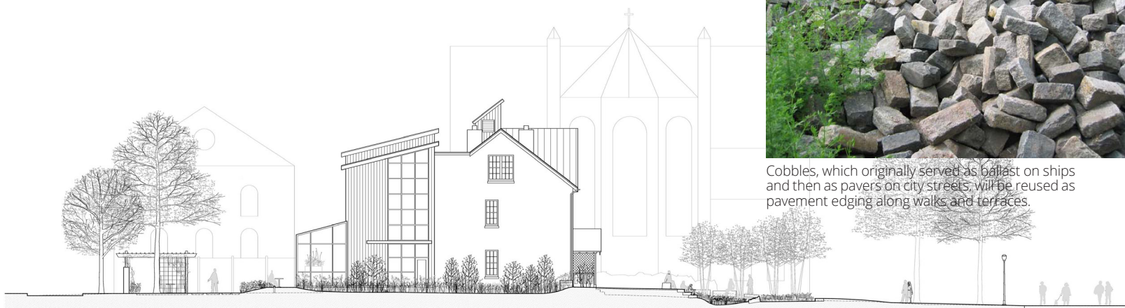
Illustrative Section through Civic House, from Irving Street to Locust Walk
